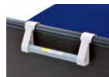
PE500-A4050 Air Mattress Hanger Material: (Bar)POM, (Hook)ABS Dimension: length 33.5cm x width 10.5cm x height 12.5cm Weight: 420g Withstand load: 10kg
